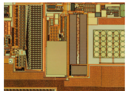
Pressure and temperature transponder ASIC. © Fraunhofer IMS
